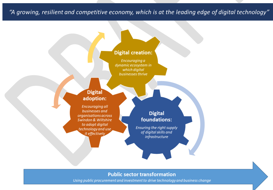
Figure 4: Strategic framework
